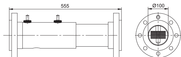
Electrolysis cell Technostar 2000 AX-F with flange connection
