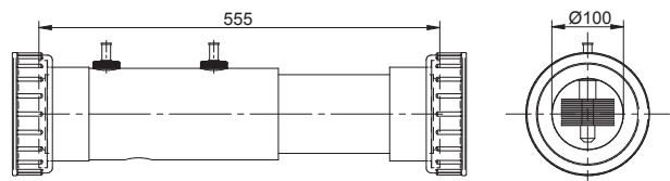
Electrolysis cell Technostar 2000 AX-G with threaded connection
