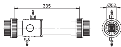
Electrolysis cell Technostar 2000 ST
